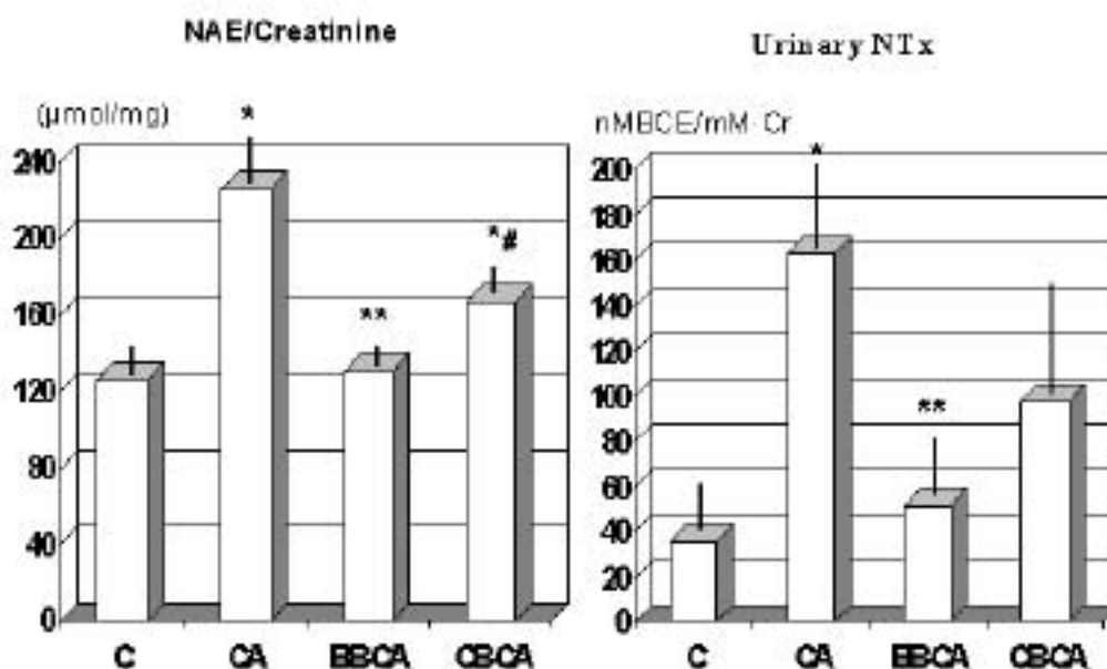
Fig. 1. Net acid excretion and urinary NTx during different alkaline supplementation in moderately exercising rats fed and high-protein diet.
